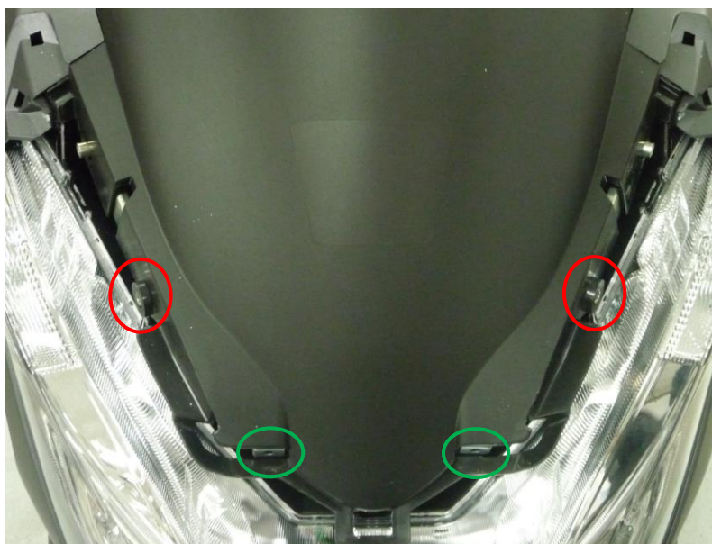
Location of the original cover fixing screws in green Location of plastic spacers in red
