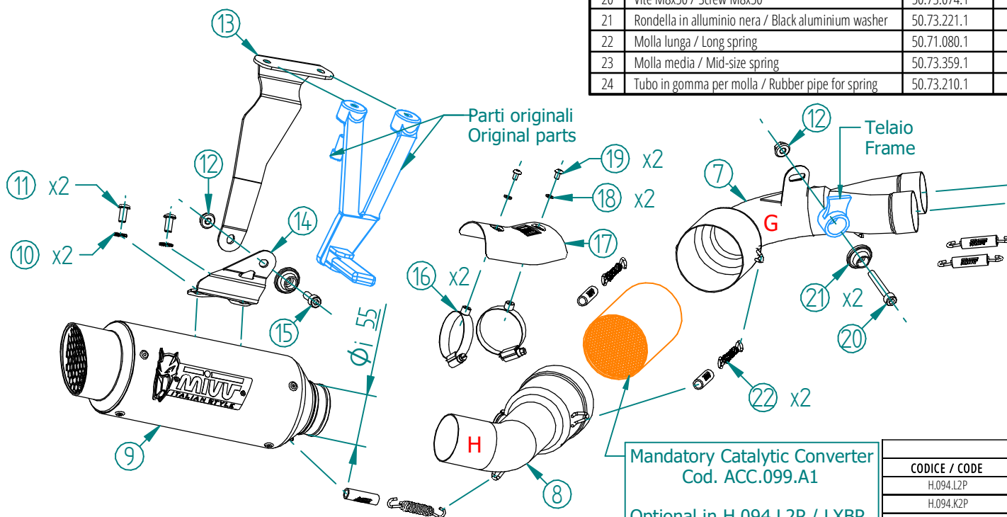
MONTAGGIO STAFFA 50.SS.1165.0 50.SS.1165.0 BRACKET ASSEMBLY
