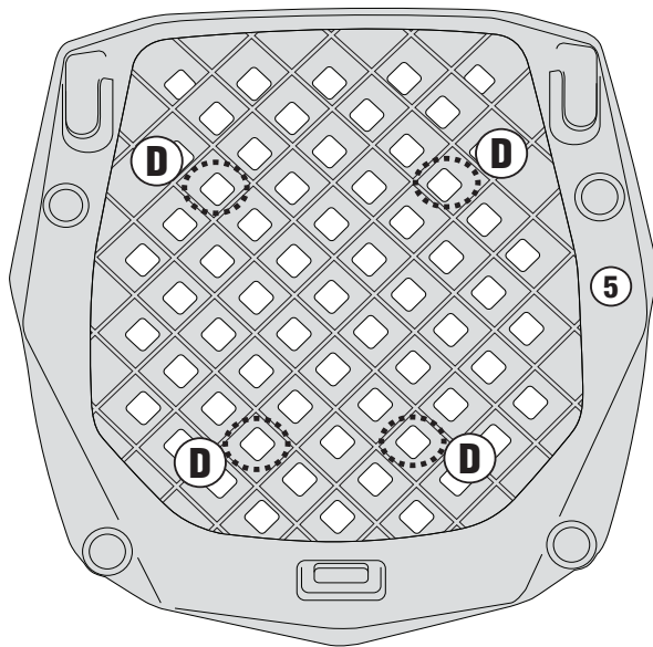
UNIVERSAL MONOKEY PLATE (E251)
